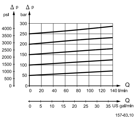
Pressure relief valve characteristic
