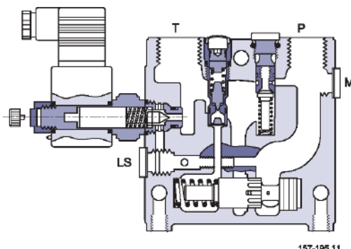
PVPX, electrical LS unloading valve
